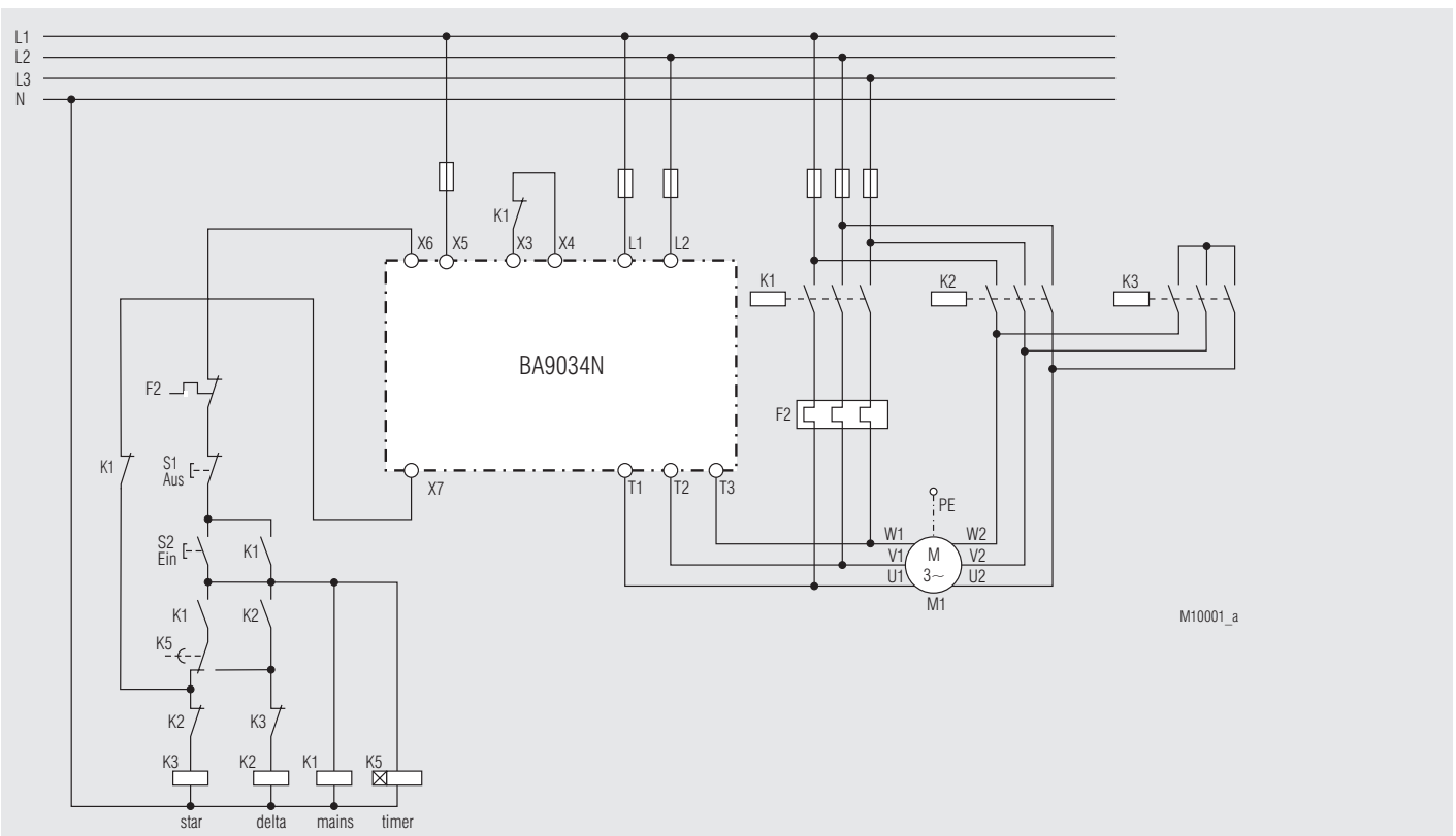
BA 9034N, 3-phasisig, \lambda - \Delta -start up
